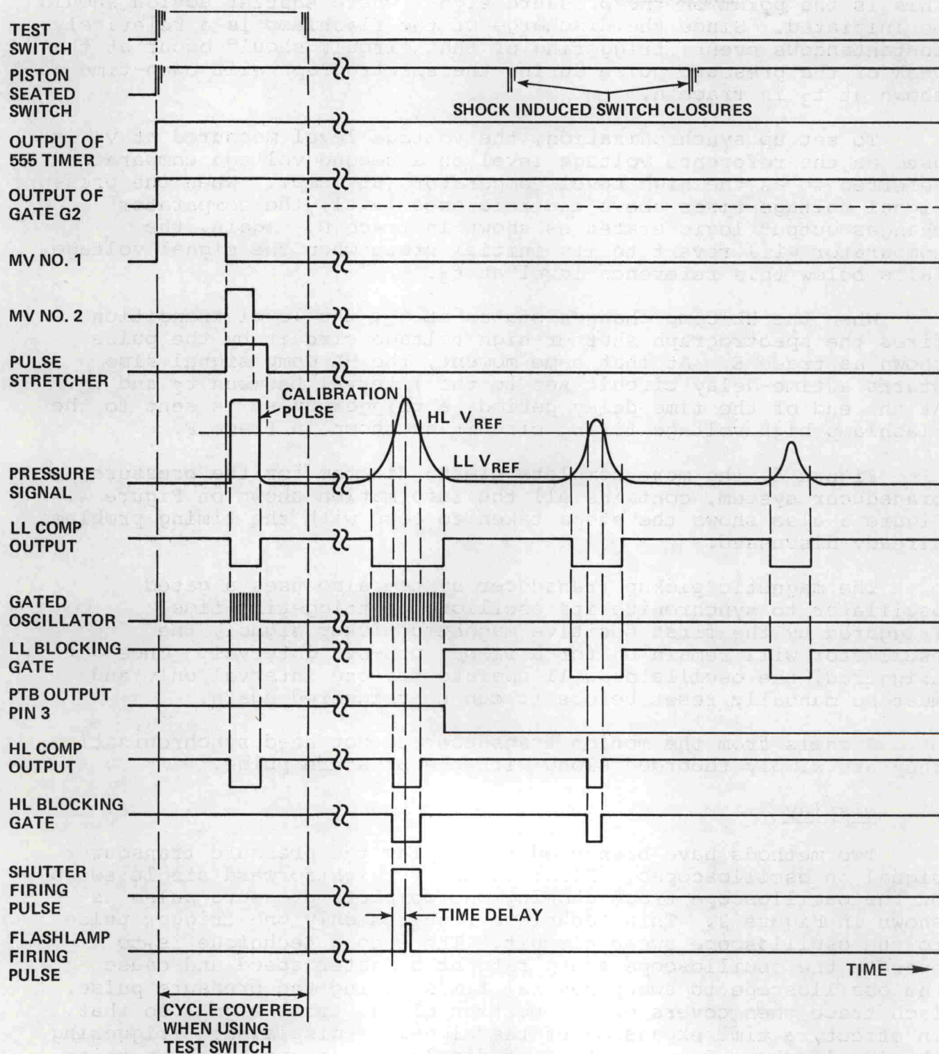
FIG. 5 PRESSURE TRANSDUCER SYSTEM TIMING DIAGRAM
